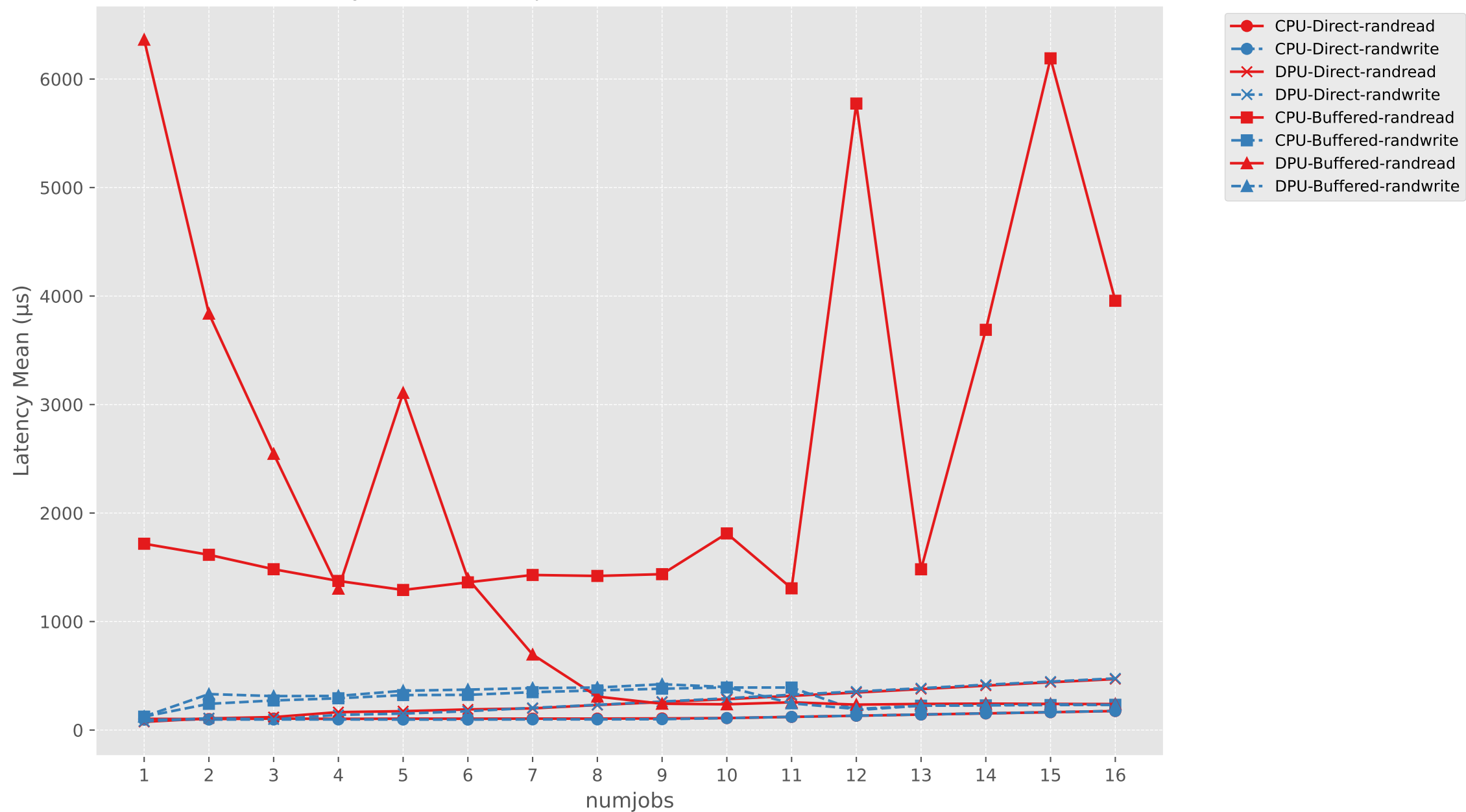
Latency Mean vs numjobs (CPU vs DPU, Direct vs Buffered)
